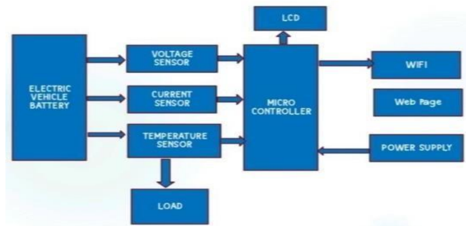
Fig. 1: Block Diagram.
